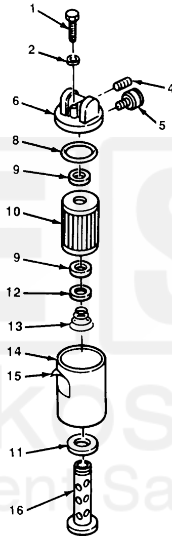
FIGURE 26. HYDRAULIC FILTER.
